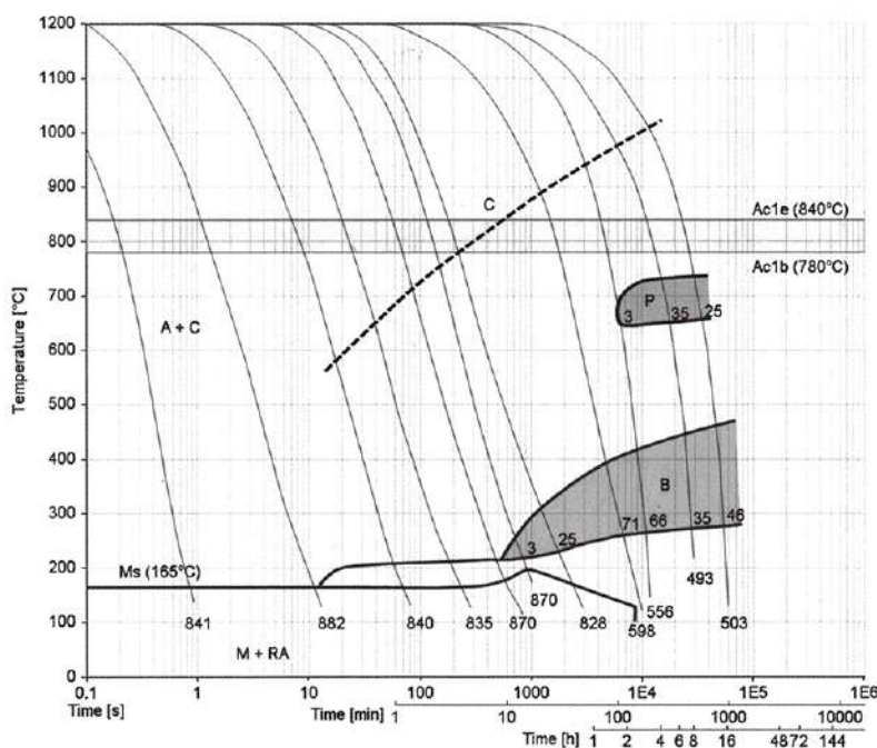
MT35 CCT GRAPH
